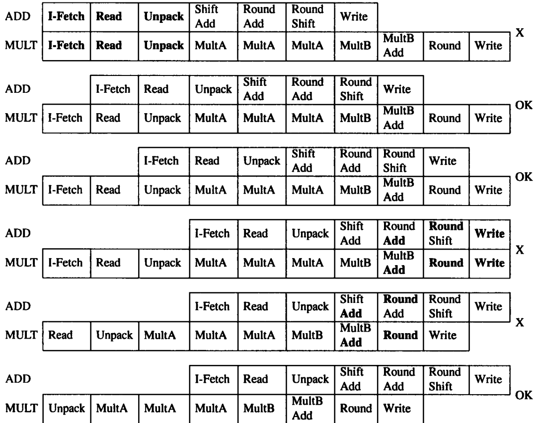
FIGURE 20.2. If there is only one functional unit of each kind, then an ADD cannot be started at the same time as a MULT (because of numerous resource hazards shown in boldface); nor three cycles after the MULT (because of Add , Round , and Write hazards); nor four cycles later (because of a Round hazard). But if there were two rounding units, then an ADD could be started four cycles after a MULT. Or with dual fetch units, multiple-access register file, and dual unpackers, the MULT and ADD could be started simultaneously.
