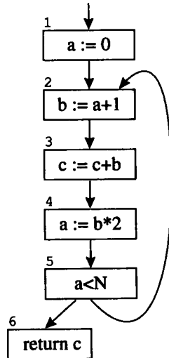
GRAPH 10.1. Control-flow graph of a program.
