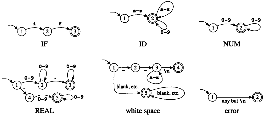
FIGURE 2.3. Finite automata for lexical tokens. The states are indicated by circles; final states are indicated by double circles. The start state has an arrow coming in from nowhere. An edge labeled with several characters is shorthand for many parallel edges.
