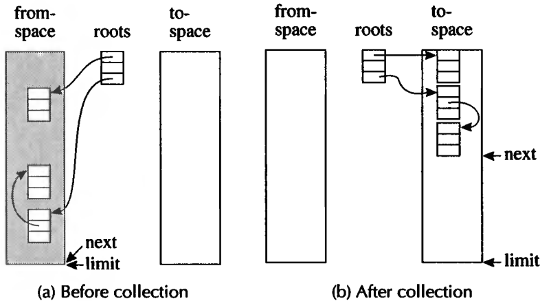
FIGURE 13.7. Copying collection.
