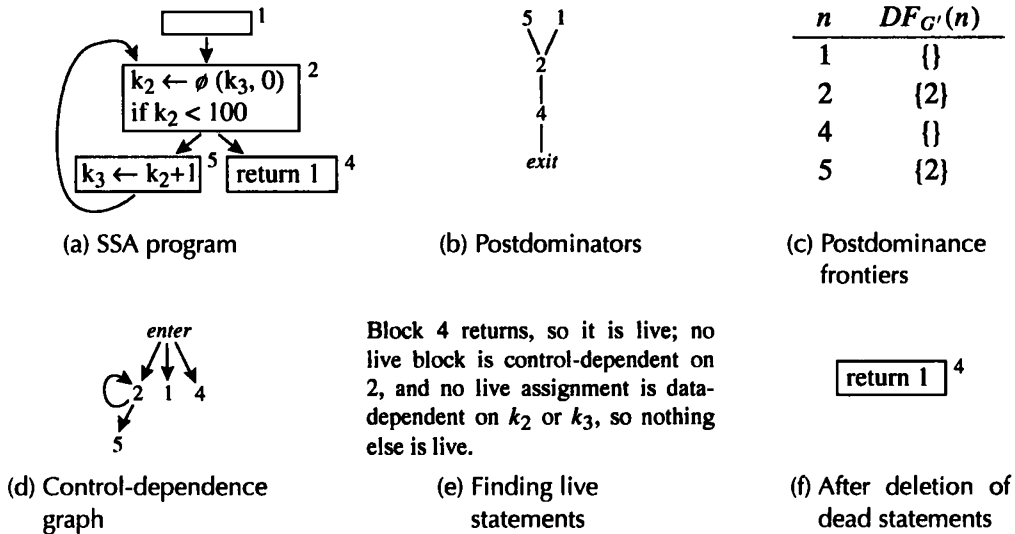
FIGURE 19.16. Aggressive dead-code elimination
