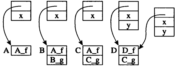
PROGRAM 14.3. Class descriptors for dynamic method lookup.
