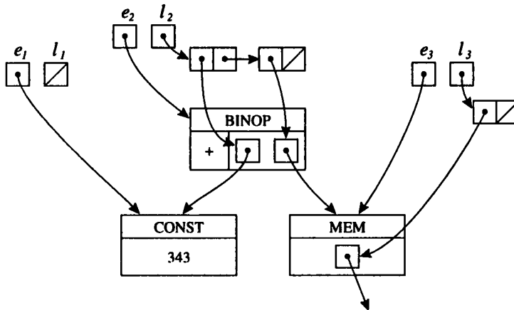
FIGURE 8.2. List-of-refs argument passed to reorder.
