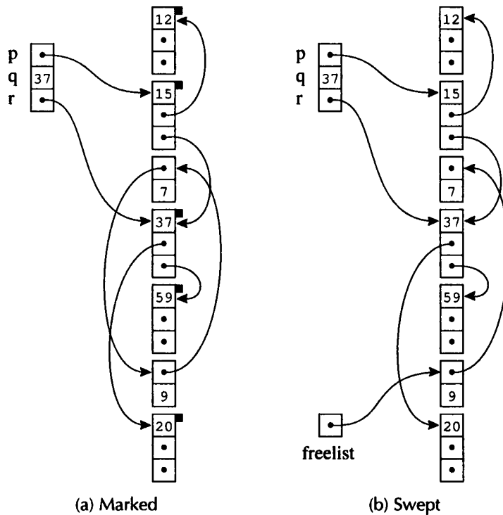
FIGURE 13.4. Mark-and-sweep collection.
