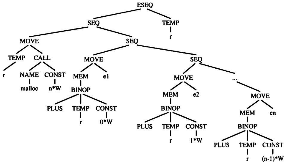
FIGURE 7.4. Record allocation.
