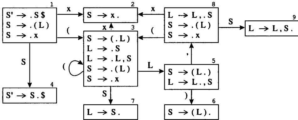
FIGURE 3.21. LR(0) states for Grammar 3.20.
